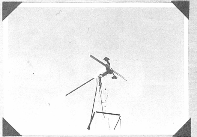
PHOTO 6. Wincharger 200 Watt - 12 Volt - Model 1222H - 1974
