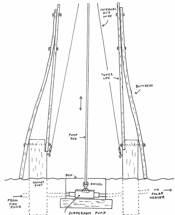
Figure 6 Sail-wing windmill with diaphragm pump.
