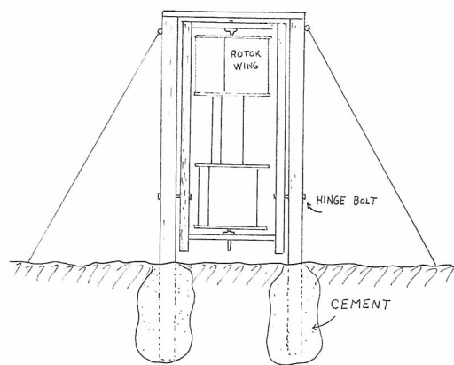
Figure 7 Savonius Rotor Tower - Rotor is Swung into Position.
