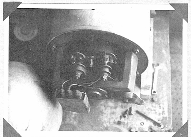
PHOTO 13. Jacobs End Bell - Showing Brushes and Capacitor
