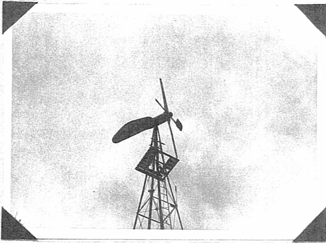
PHOTO 17. Air Electric 3000 Watt - 32 Volt - Paddle type Governor
