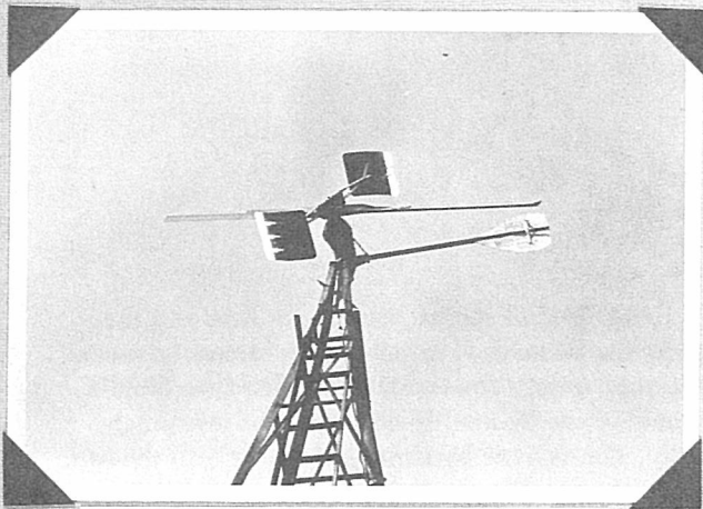
PHOTO 2. Wincharger 1200 Watt - 32 Volt - Model 3214 - 1940
