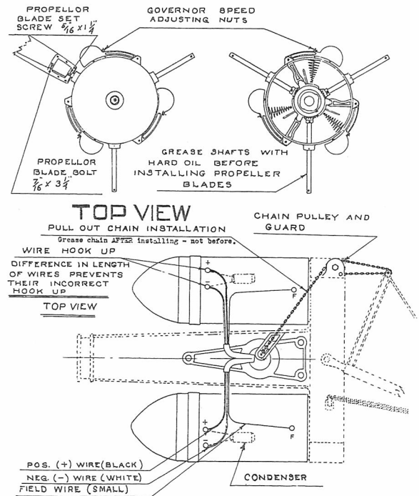
FIGURE B Jacobs Twin-Motor 1500 Watt - 32 Volt - Model 15
