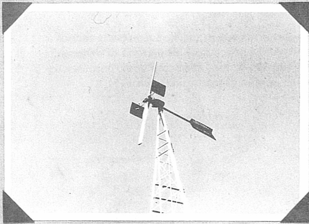
PHOTO 1. Wincharger 650 Watt - 32 Volt - Model 321 - 1936
