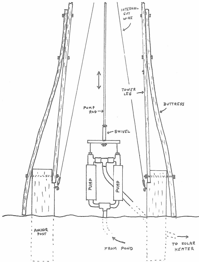
Figure 4 Sail-wing windmill with buttresses and two pumps.
