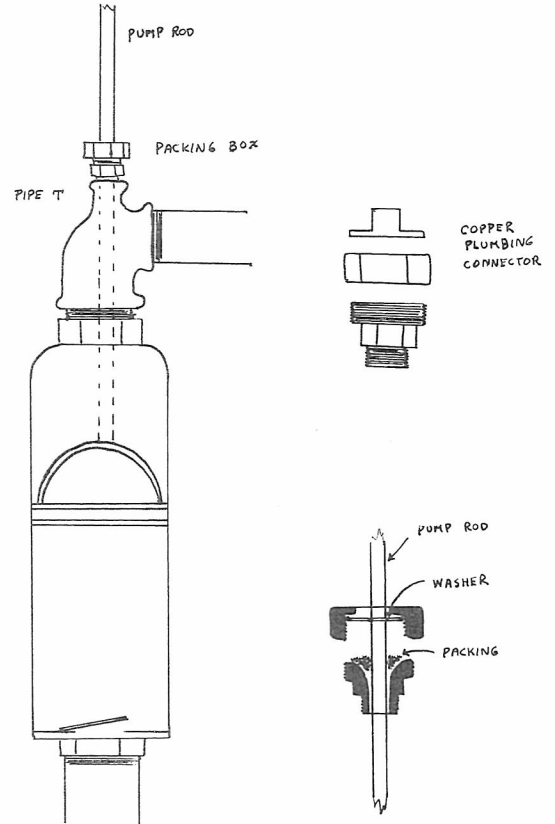
Figure 5 Inexpensive packing box for piston pump.
