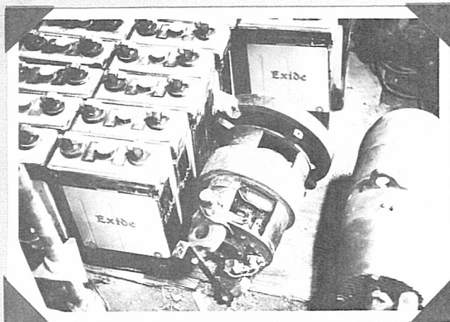
PHOTO 16. Air Electric 2000 Watt - 32 Volt - Generator Against Batteries
