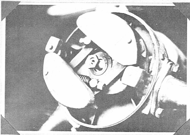
PHOTO 11. Rurallite Governor - Showing Flyball Weights
