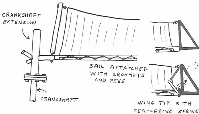
Figure 2 Advanced sail-wing details.
