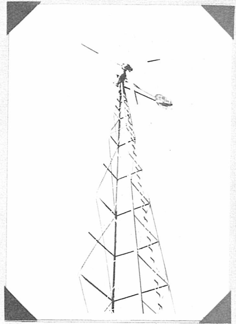
PHOTO 12. Jacobs 2500 Watts - 110 Volts - 1950
